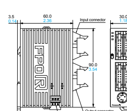
<Reference measuring for wiring>
