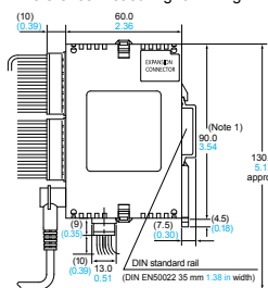
<Reference measuring for wiring>
