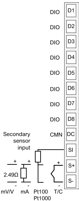
PV INPUT 8 x DIGITAL IN / OUT
