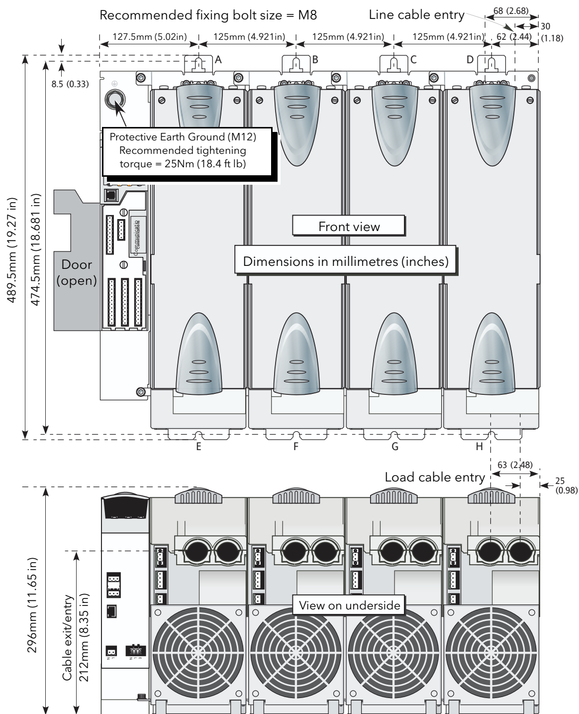
Figure 5) 500A/630A units
