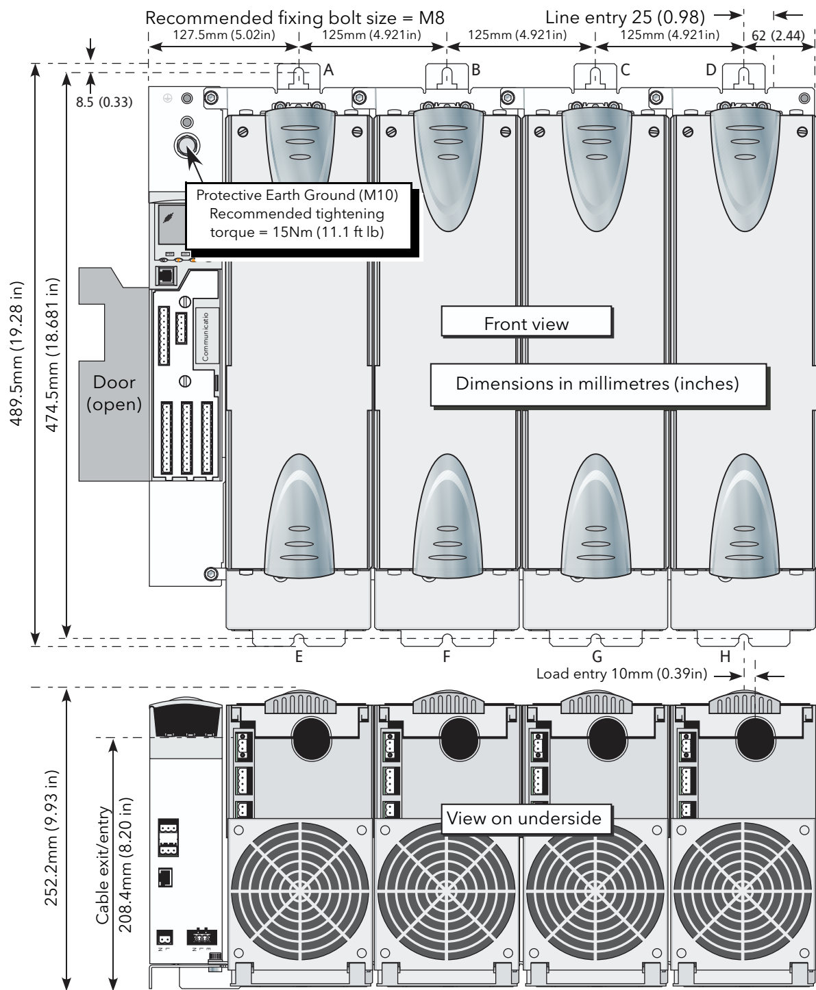
Figure 4) 400A unit
