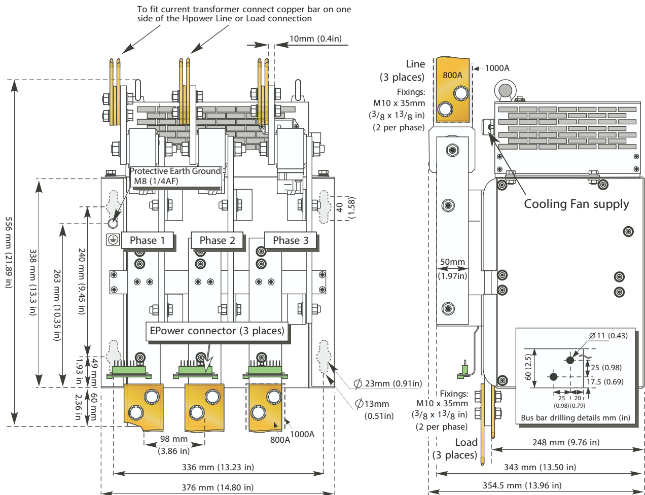
Figure 8) Thyristor stack - 800A/1000A, 3 phase units
