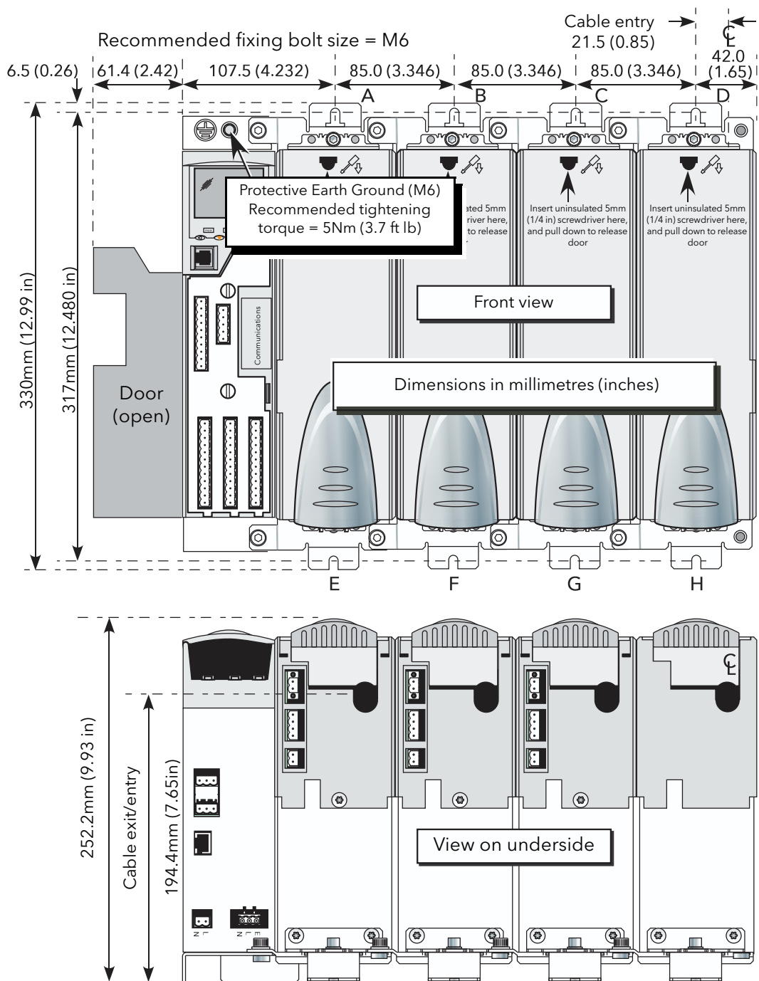
Figure 1) 50A/100A units
