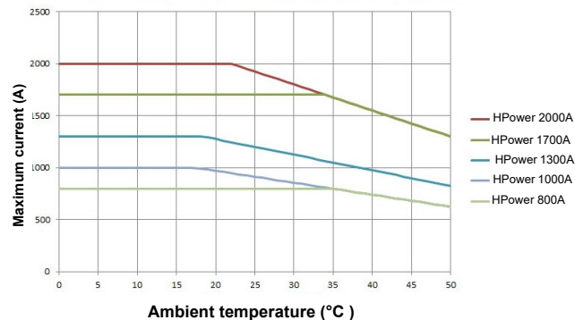
Derating curve at 2000m altitude with fan supply at nominal voltage -15%
