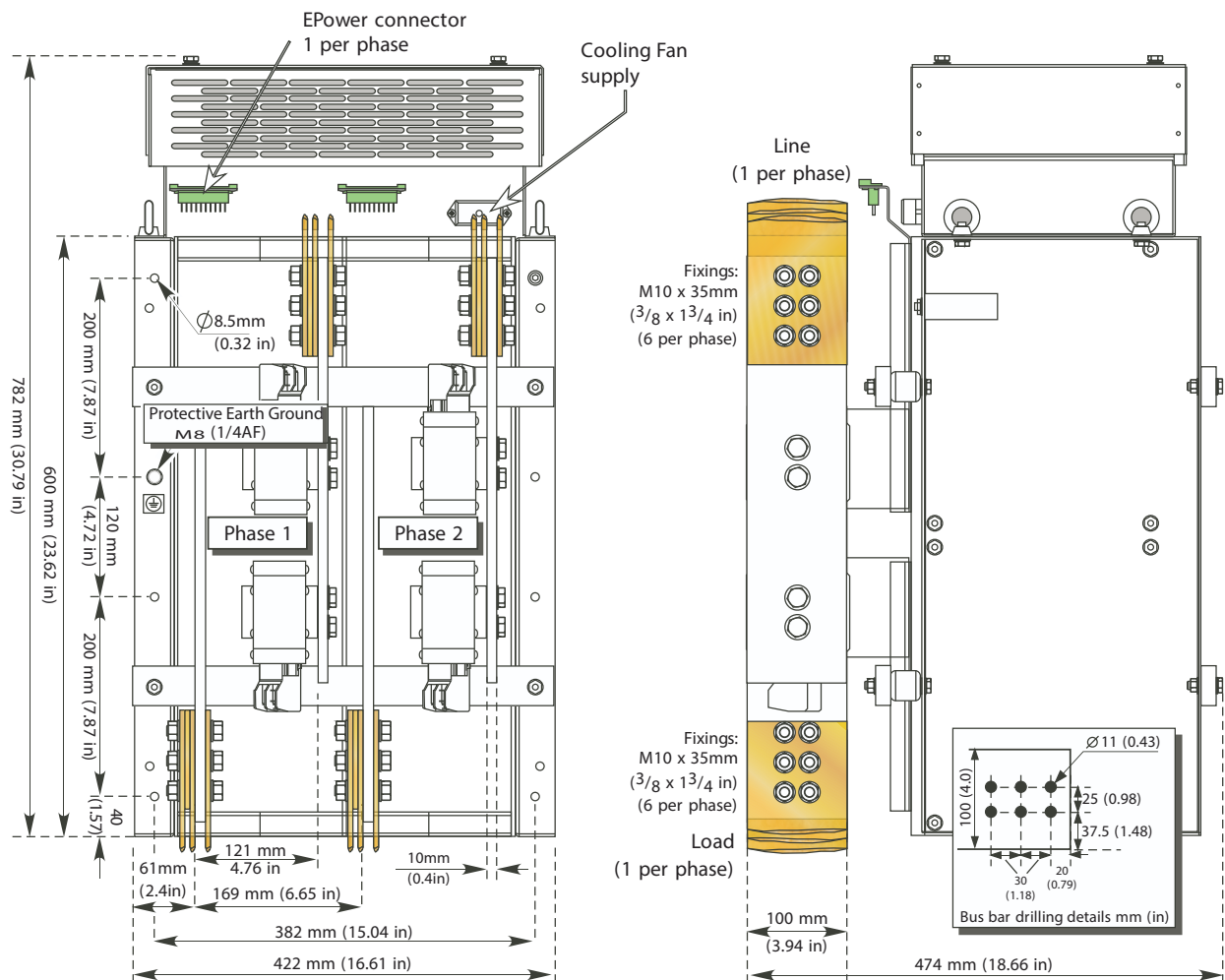
Figure 10) Thyristor stack - 1700A/2000A air cooled 1 or 2 phase units
