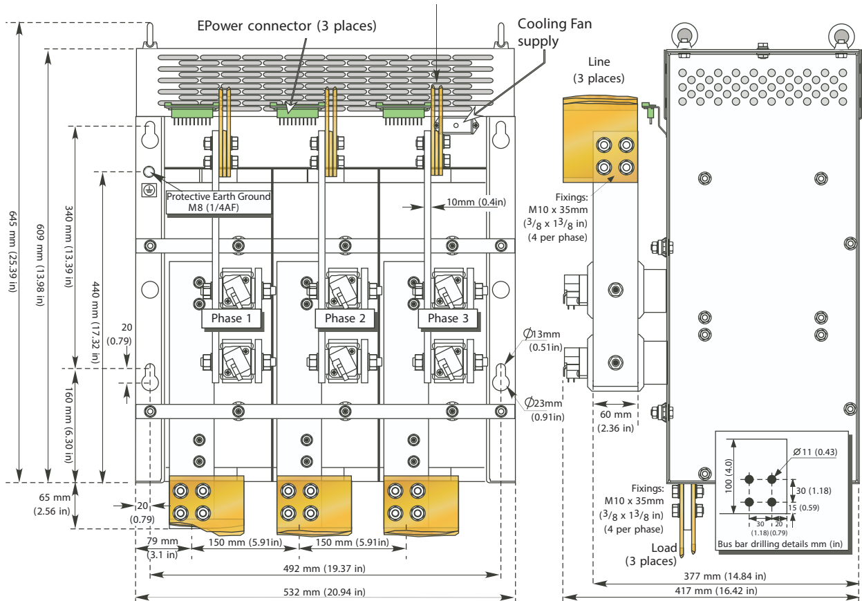
Figure 9) Thyristor stack - 1300A 3 phase units
