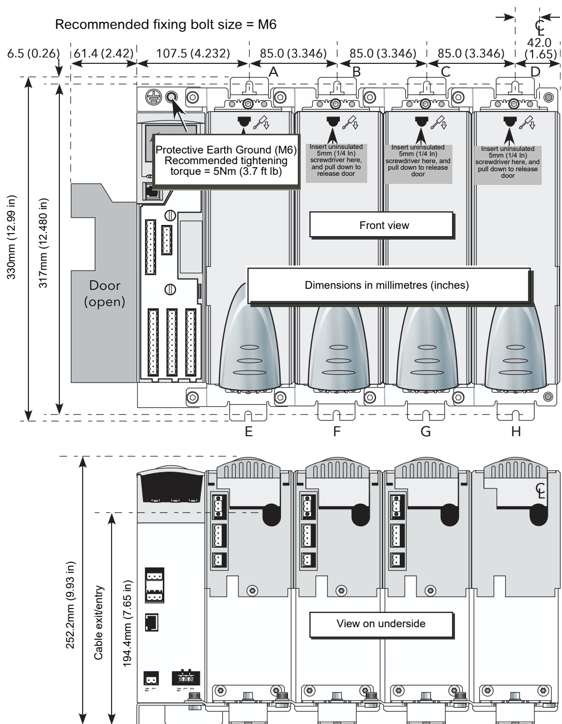
Figure 6) Fixing details (EPower MC units)
