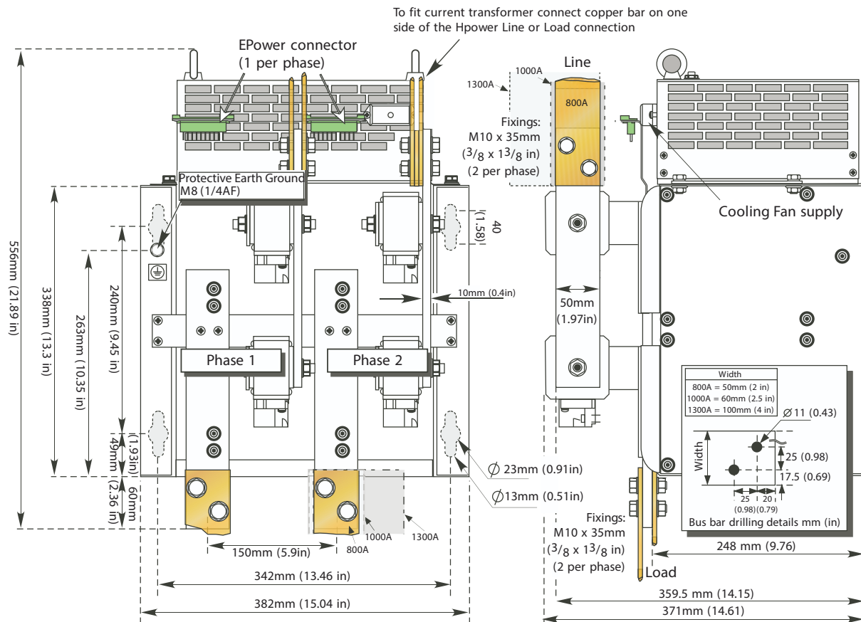
Figure 7) Thyristor stack - 800A/1000A/1300A, 1 or 2 phase units
