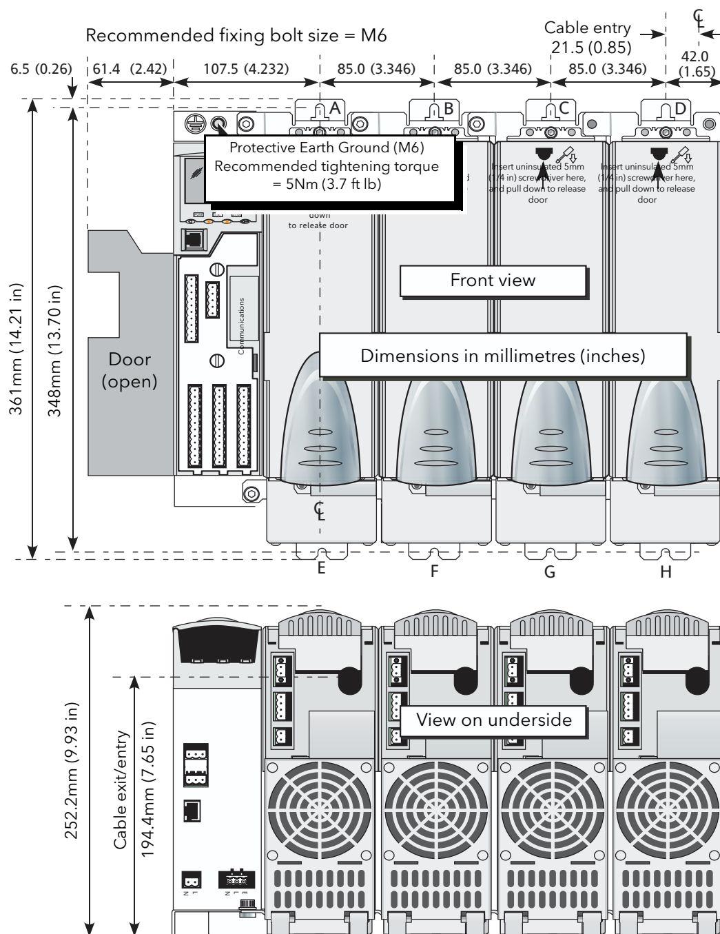
Figure 2) 160A unit
