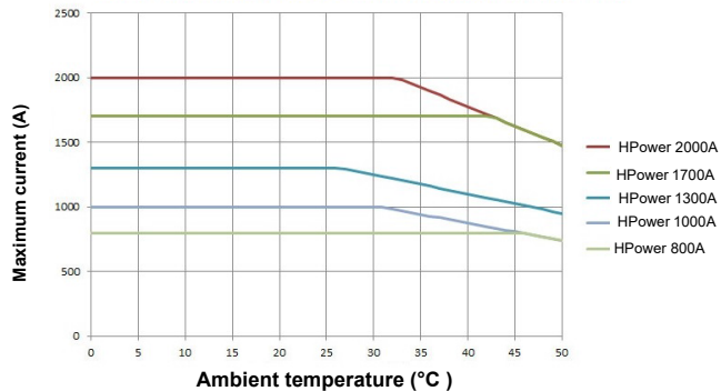
Derating curve at 1000m altitude with fan supply at nominal voltage -15%
