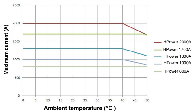
Derating curve at 1000m altitude with fan supply at nominal voltage
