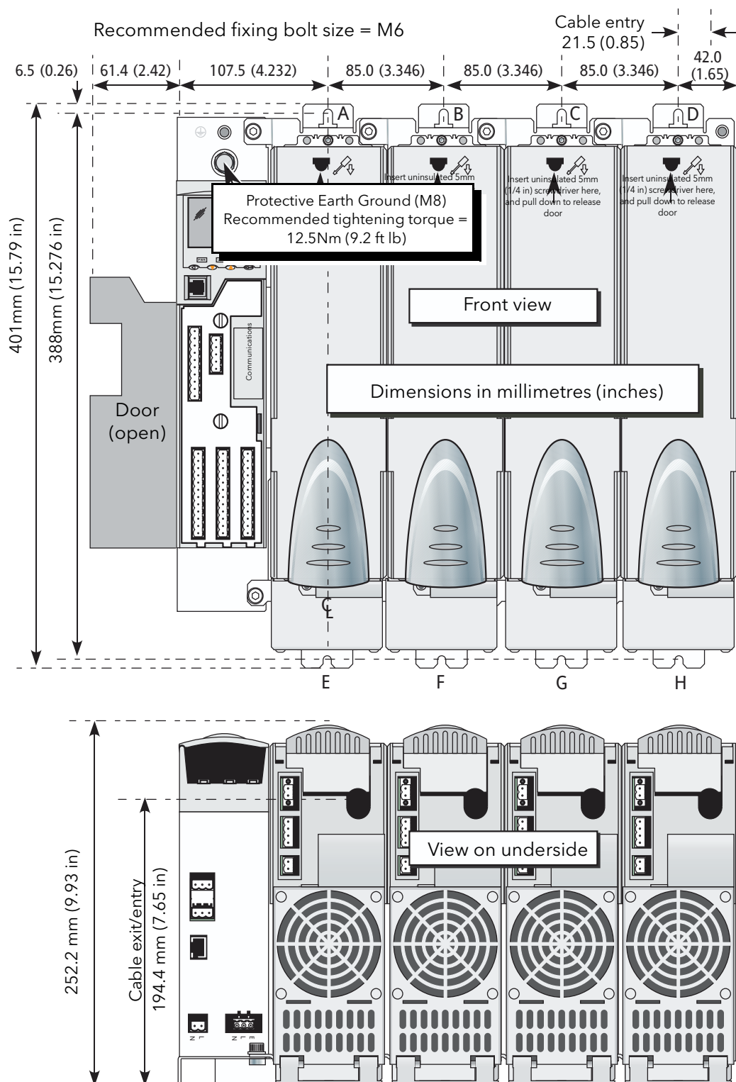
Figure 3) 250A unit
