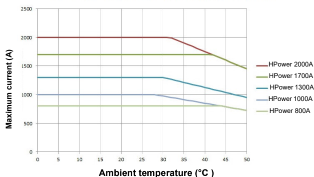
Derating curve at 2000m altitude with fan supply at nominal voltage
