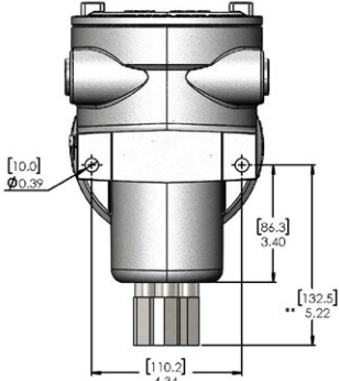
**4.27 [108.5] WEATHERPROOF VERSION
