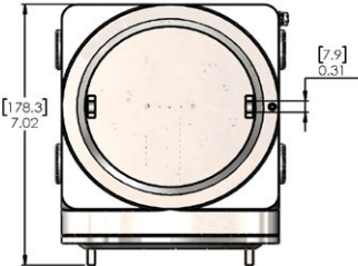
*9.11 [231.4] WEATHERPROOF VERSION
