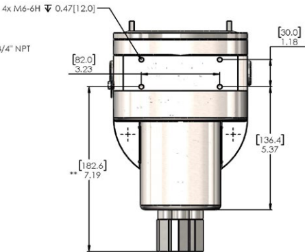
**6.24 [158.5] WEATHERPROOF VERSION
