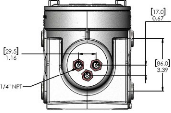
**4.27 [108.5] WEATHERPROOF VERSION
