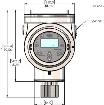
*9.11 [231.4] WEATHERPROOF VERSION
