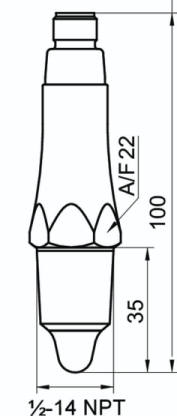
1/2-14 NPT (BCID: N02)
