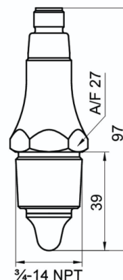
3/4-14 NPT (BCID: N03)
